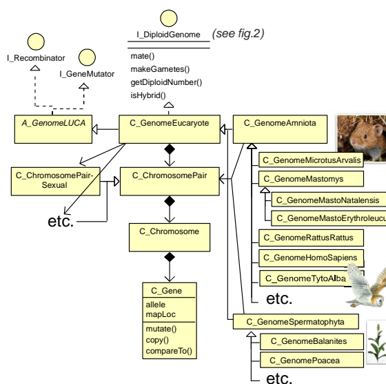
Figure 3: UML-based class diagram of the genetic part of the model, as obtained from the case studies. Left: Genetic structure allowing the transmission of the genetic heritage of a simulated agent to its ‘progeny’ following mating. The structure of the tree on the right-hand site resembles a knowledge base for instantiating, in the general scheme, any type of species (rodent, predator, man, etc.) and its characteristics (life expectancy, age at maturity, etc.). Legend: identical to Figure 2, LUCA: last universal common ancestor, the root of the species phylogeny (Forterre et al. , 2005).
